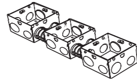
3 Gang Switch & Socket GI Box
